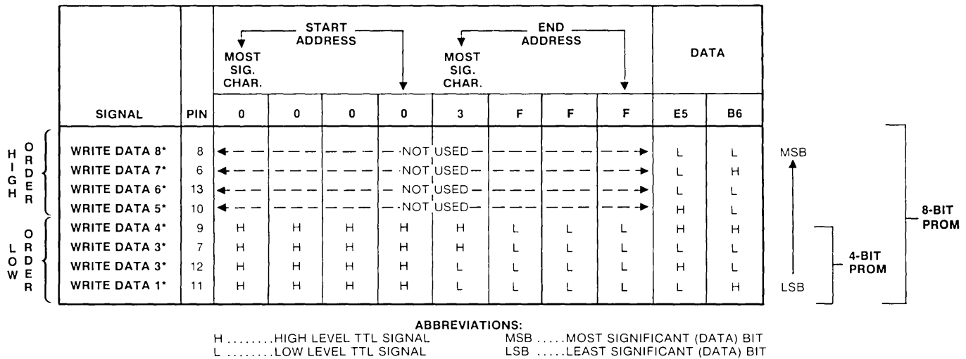
PARALLEL I/O WRITE DATA SIGNALS FOR ADDRESS FIELD DEFINITION AND DATA TO BE PROGRAMMED
