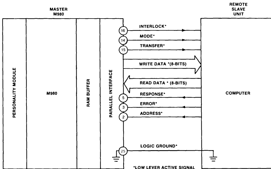
M980 Configured as a Master Controller
