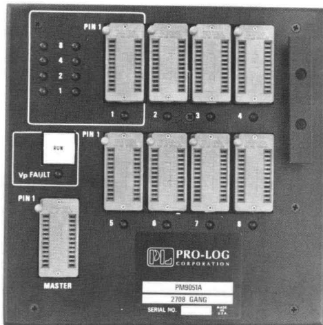
Gang Personality Module
