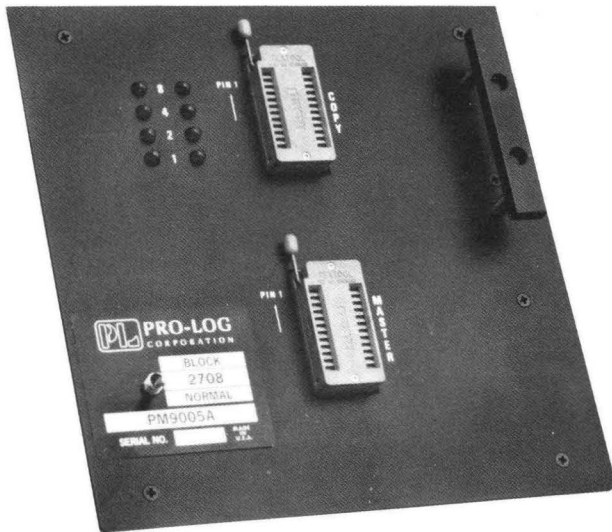
Dedicated Personality Module
