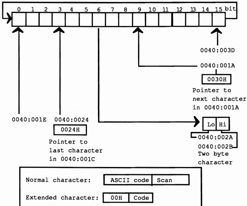
Keyboard buffer with start and end pointers
