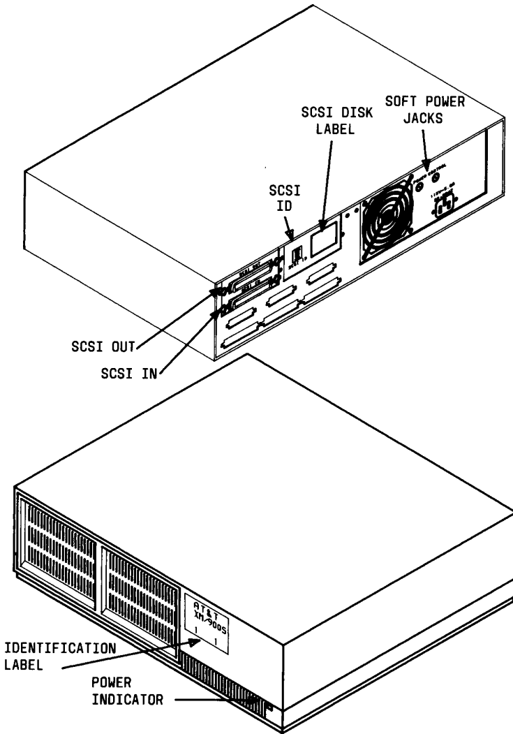
Figure 2-4: SCSI Expansion Module (XM/900S)
