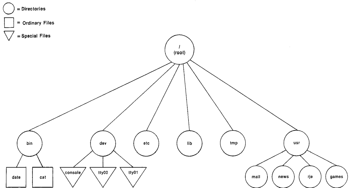
Figure 3-1. Sample file system
