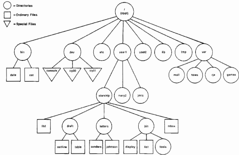
3-7 Figure 3-2. A directory that organizes home directories is equivalent to directories like bin and tmp in the file system
