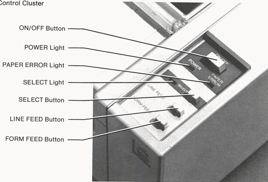
Figure 1-8. Control Cluster
