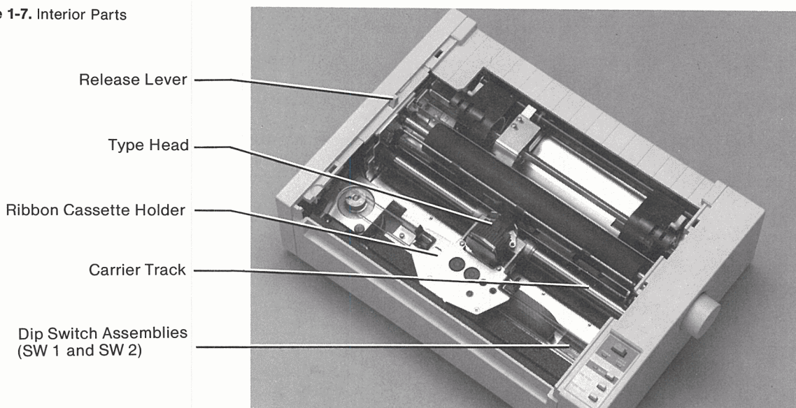
Figure 1-7. Interior Parts
