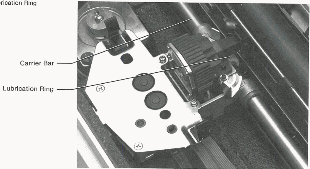
Figure 3-3. Lubrication Ring
