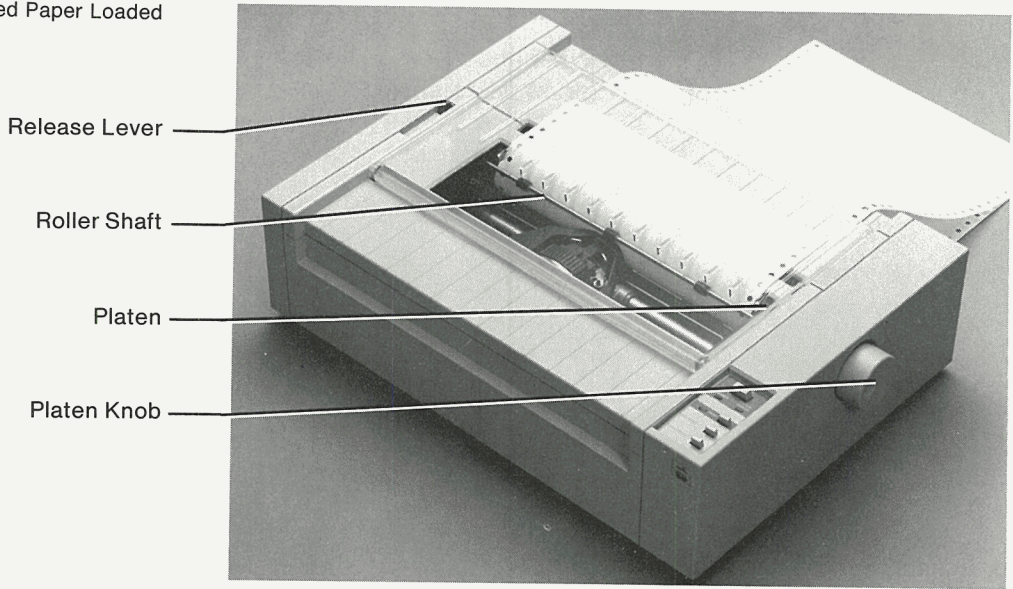
Figure 2-5. Pin-Feed Paper Loaded
