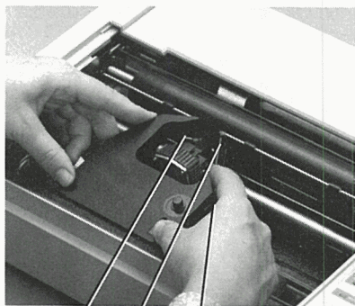
Cassette Support Ribbon Guide Plate Ribbon Guide
