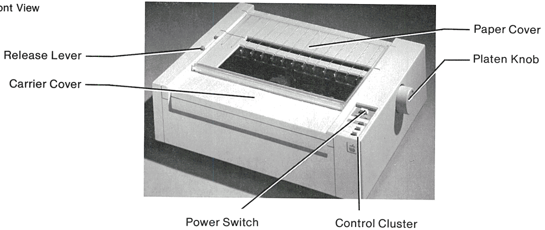
Figure 1-3. Front View
