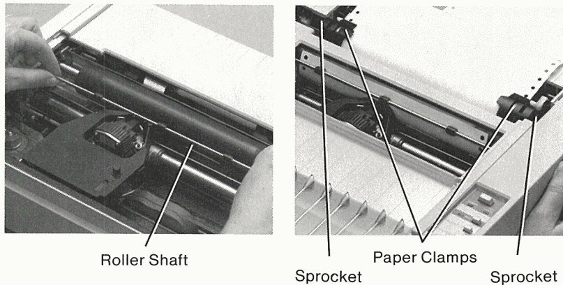
Figure 2-4. Loading Pin-Feed Paper
