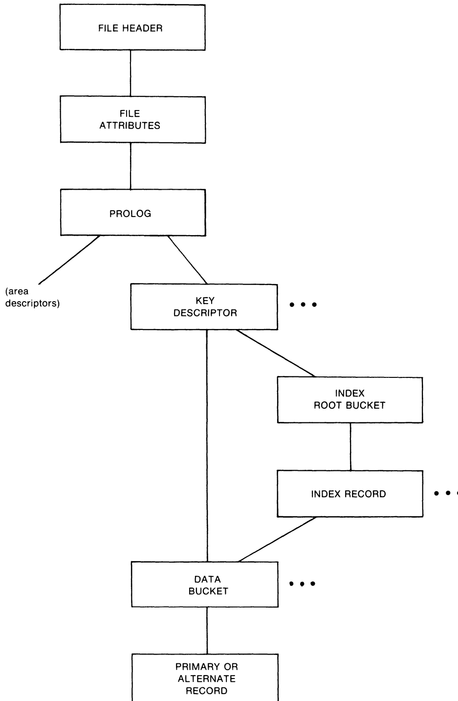
Figure ARMS-4 KEY DESCRIPTOR Path
