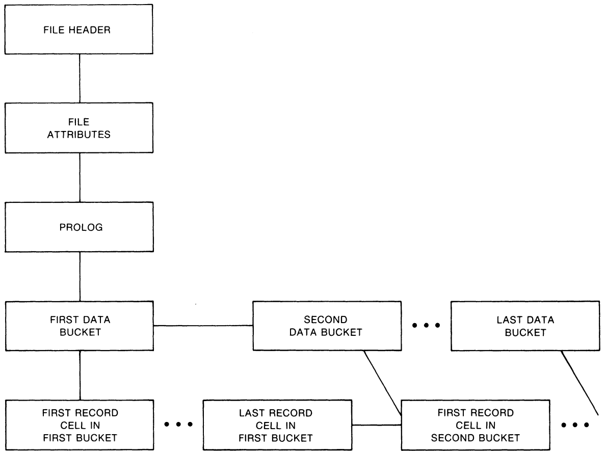
Figure ARMS-2 Structure of Relative Files
