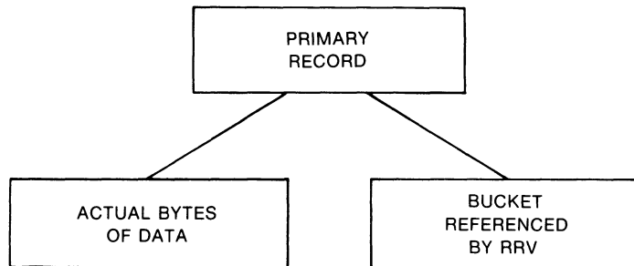
Figure ARMS-5 Structure of Primary Records
