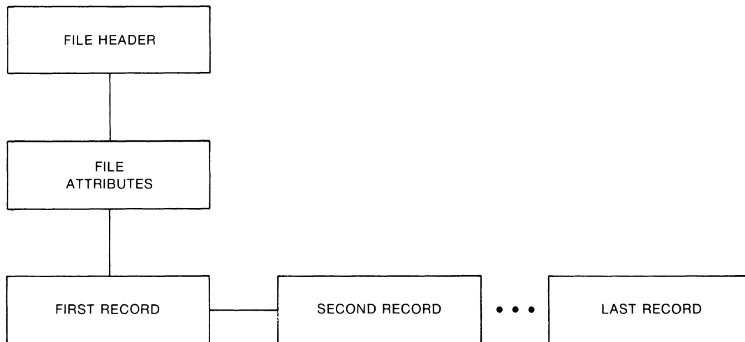
Figure ARMS-1 Structure of Sequential Files
