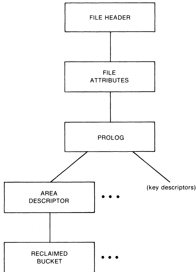
Figure ARMS-3 AREA DESCRIPTOR Path
