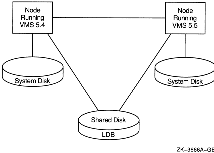
Figure 2-2 Invalid Mixed Version VAXcluster with Shared License Database
