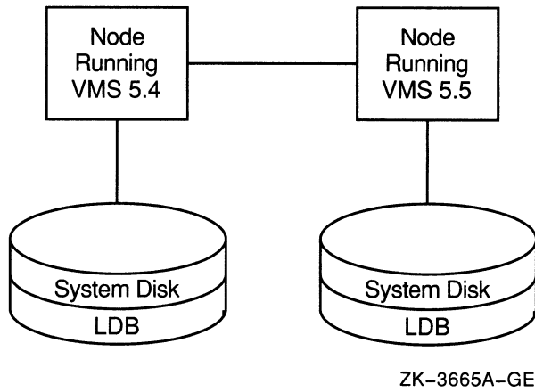
Figure 2-1 Valid Mixed Version VAXcluster with Separate License Databases
