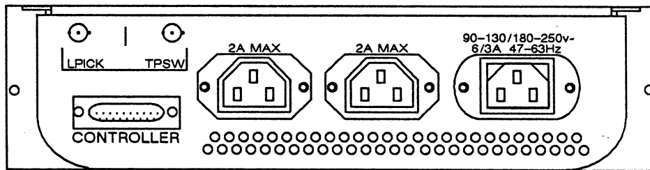
Figure 2. Backside Connectors for the Peripheral Multiplexers
