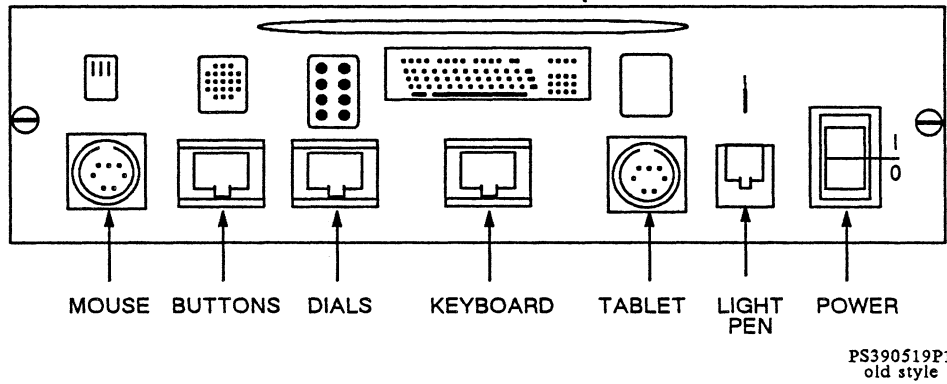
Figure 3. Multiplexer Connectors for the PS 300
