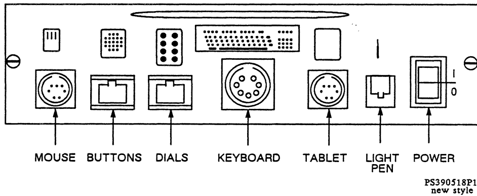
Figure 4. Multiplexer Connectors for the LC Peripherals
