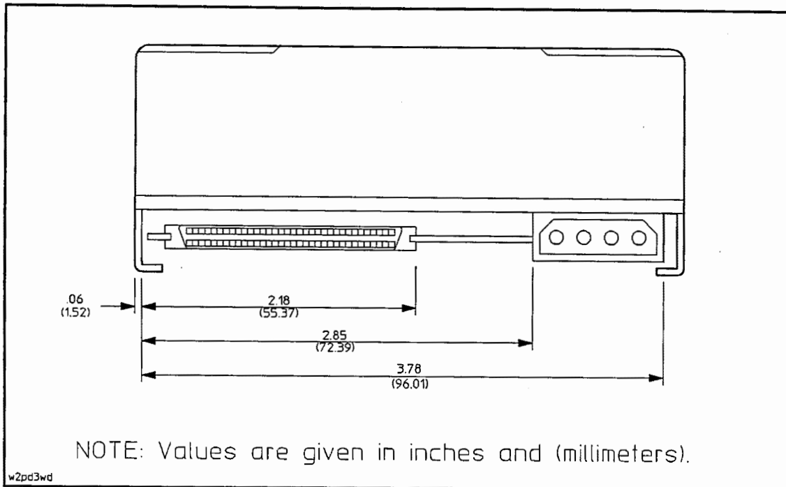
Figure G-3. Wide, Differential: Connector Dimensions
