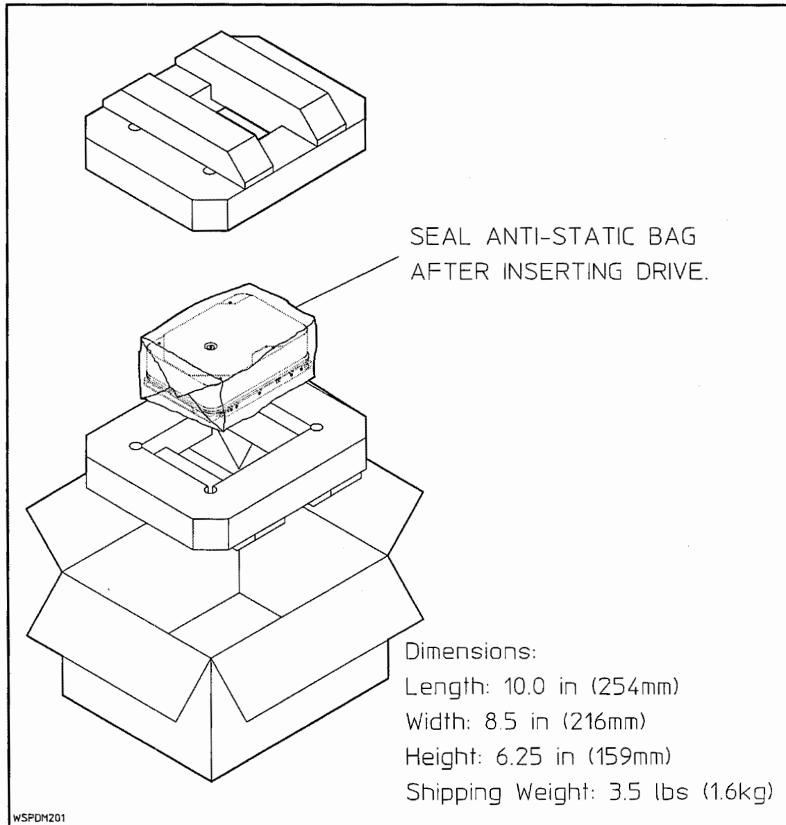
Figure 2-1. Single-Unit Packaging
