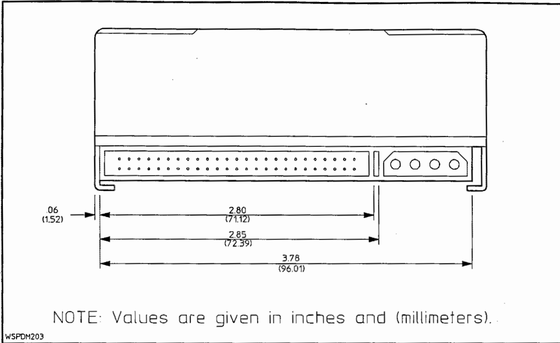
Figure E-3. Narrow, Single-Ended: Connector Dimensions
