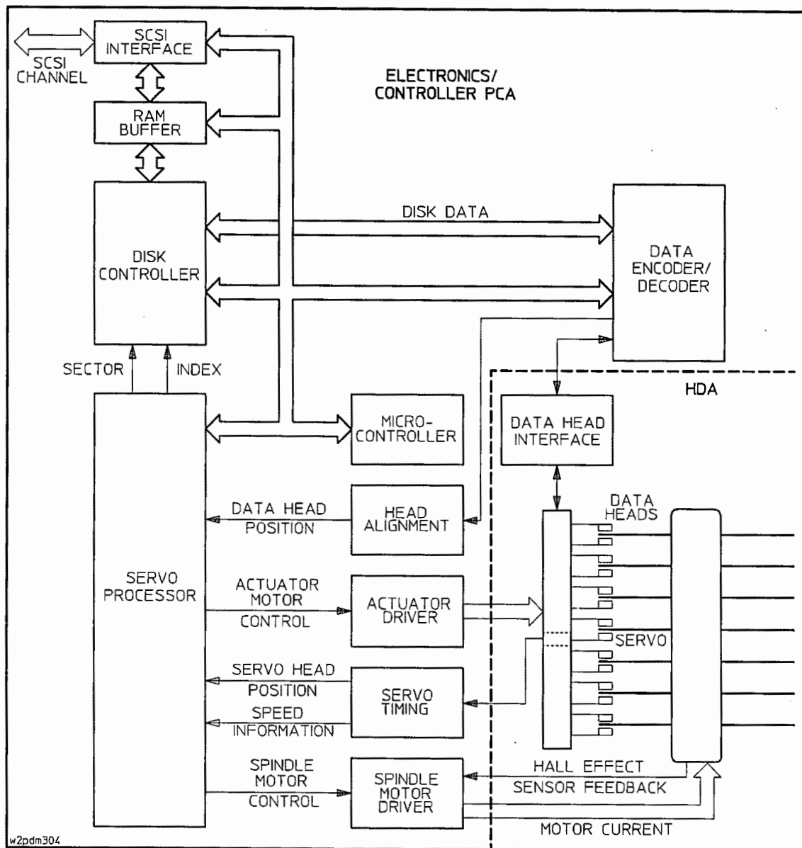
Figure 3-3. Disk Drive Block Diagram
