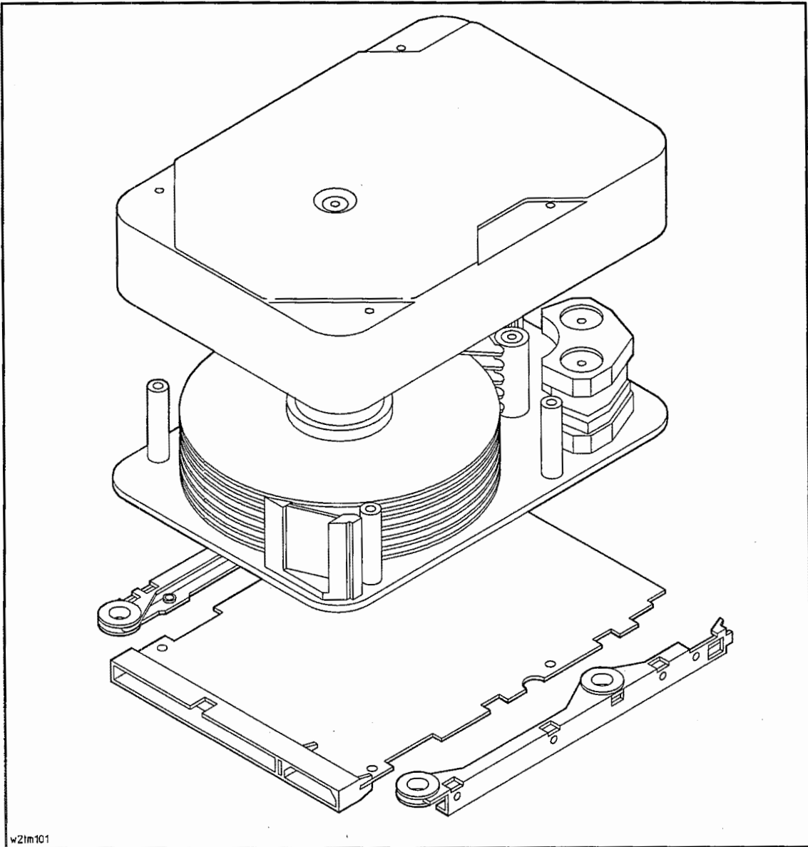
Figure 1-1. Disk Drive Major Components
