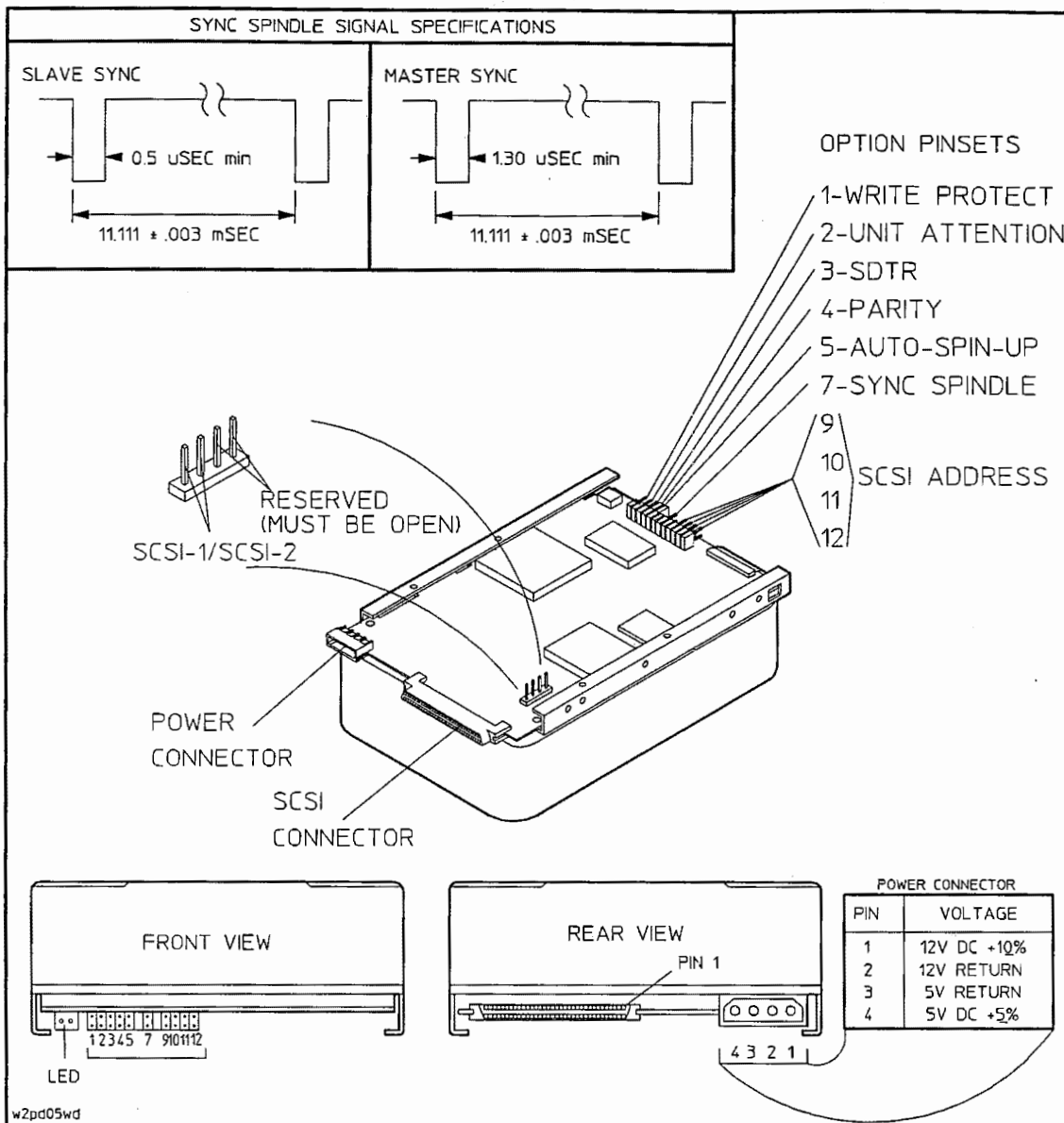
Figure G-2. Wide, Differential: Interface, Address and Option Connectors
