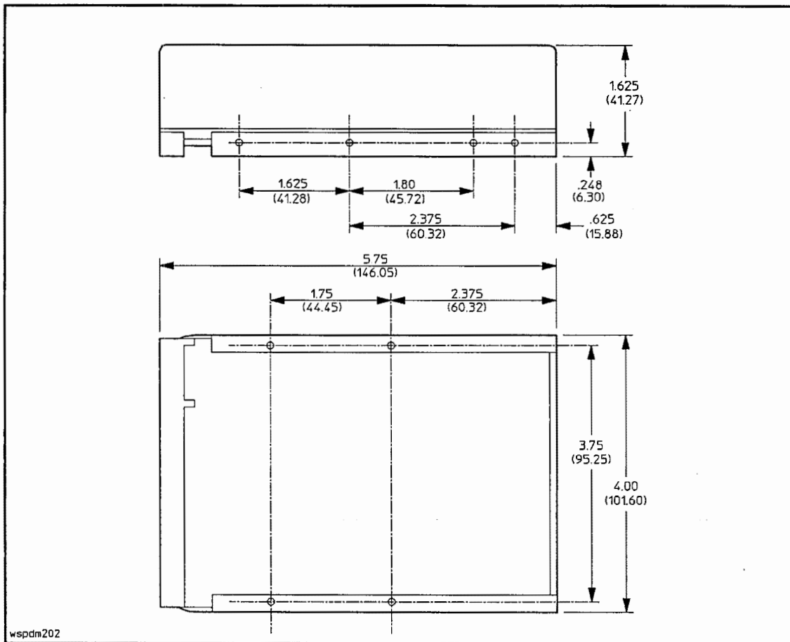
Figure E-1. Narrow, Single-Ended: Disk Drive Dimensions and Mounting Locations
