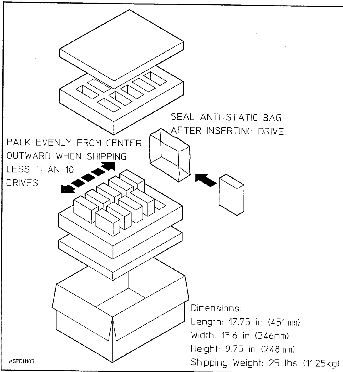
Figure 2-2. Ten-Unit Packaging
