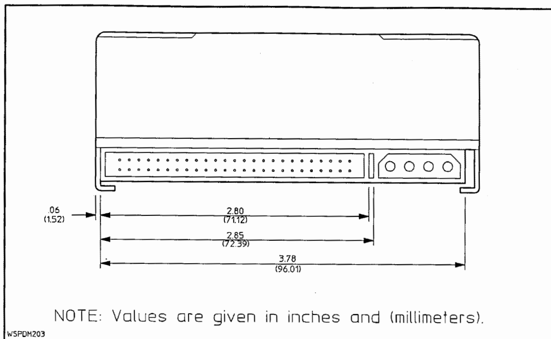
Figure F-3. Narrow, Differential: Connector Dimensions
