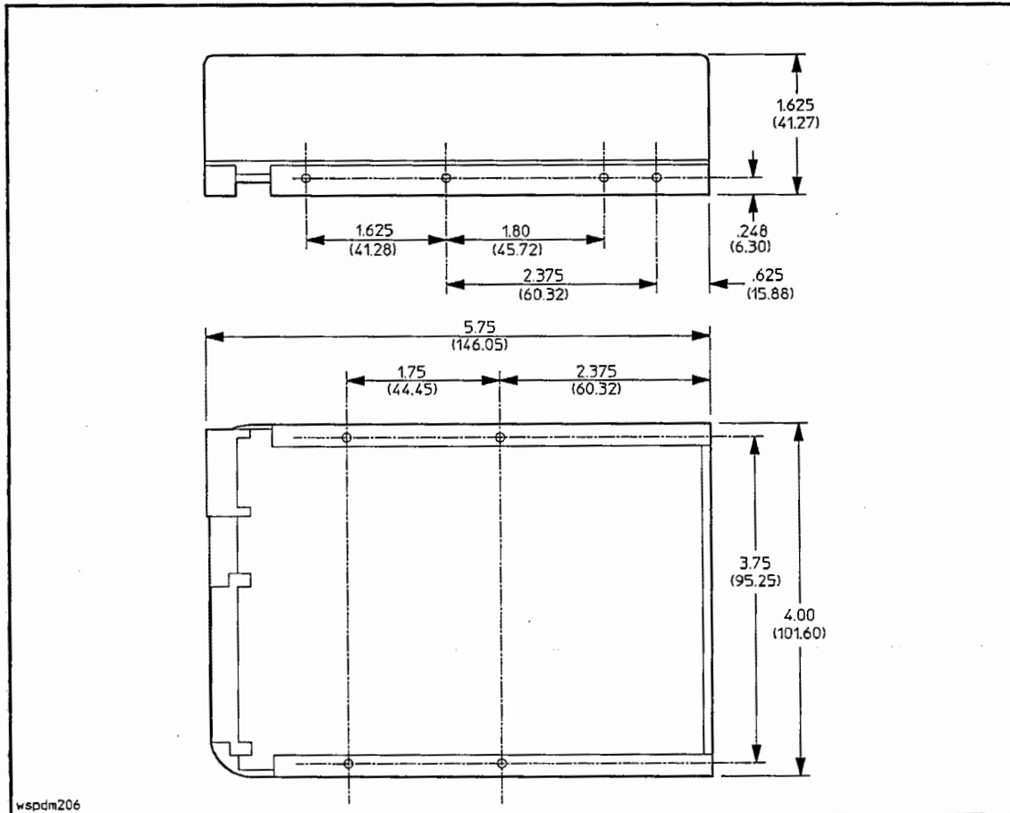
Figure G-1. Wide, Differential: Disk Drive Dimensions,
