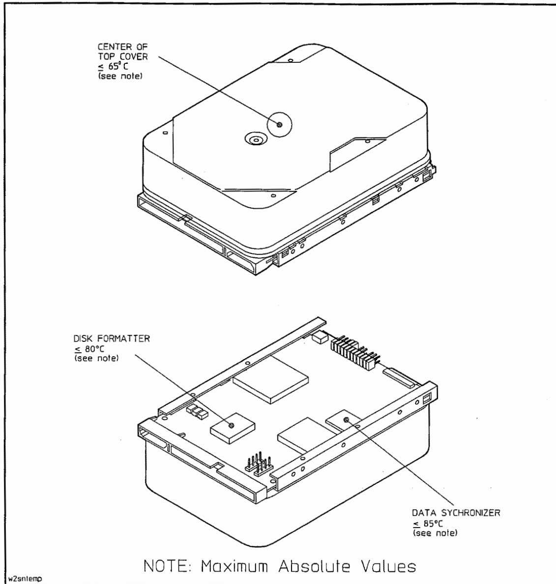
Figure E-4. Narrow, Single-Ended: Operating Temperatures
