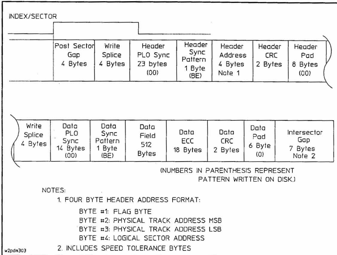
Figure 3-2. Formatted Physical Sector Allocation
