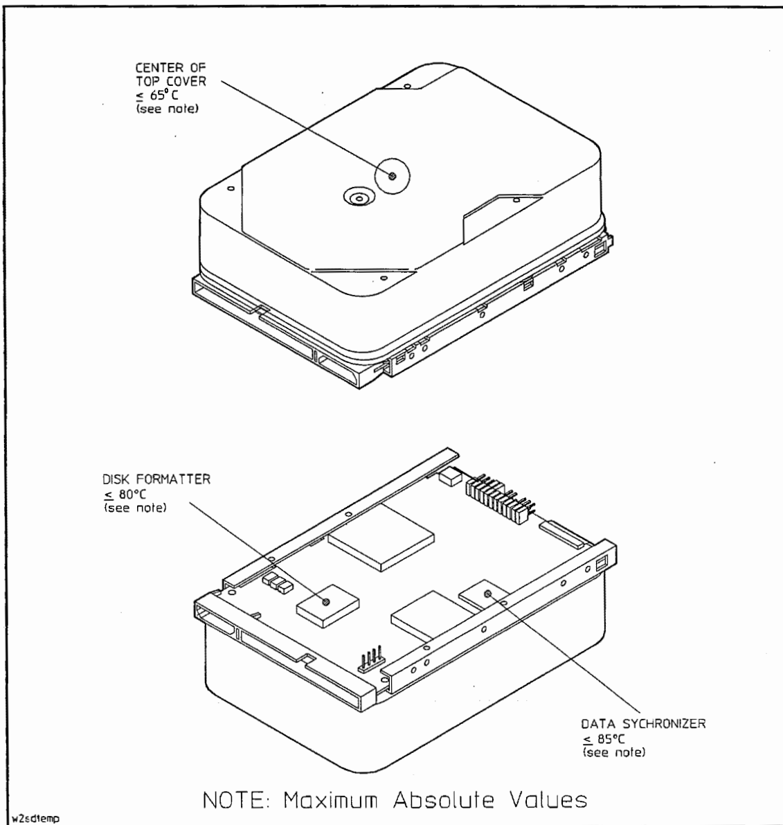
Figure F-4. Narrow, Differential: Operating Temperatures
