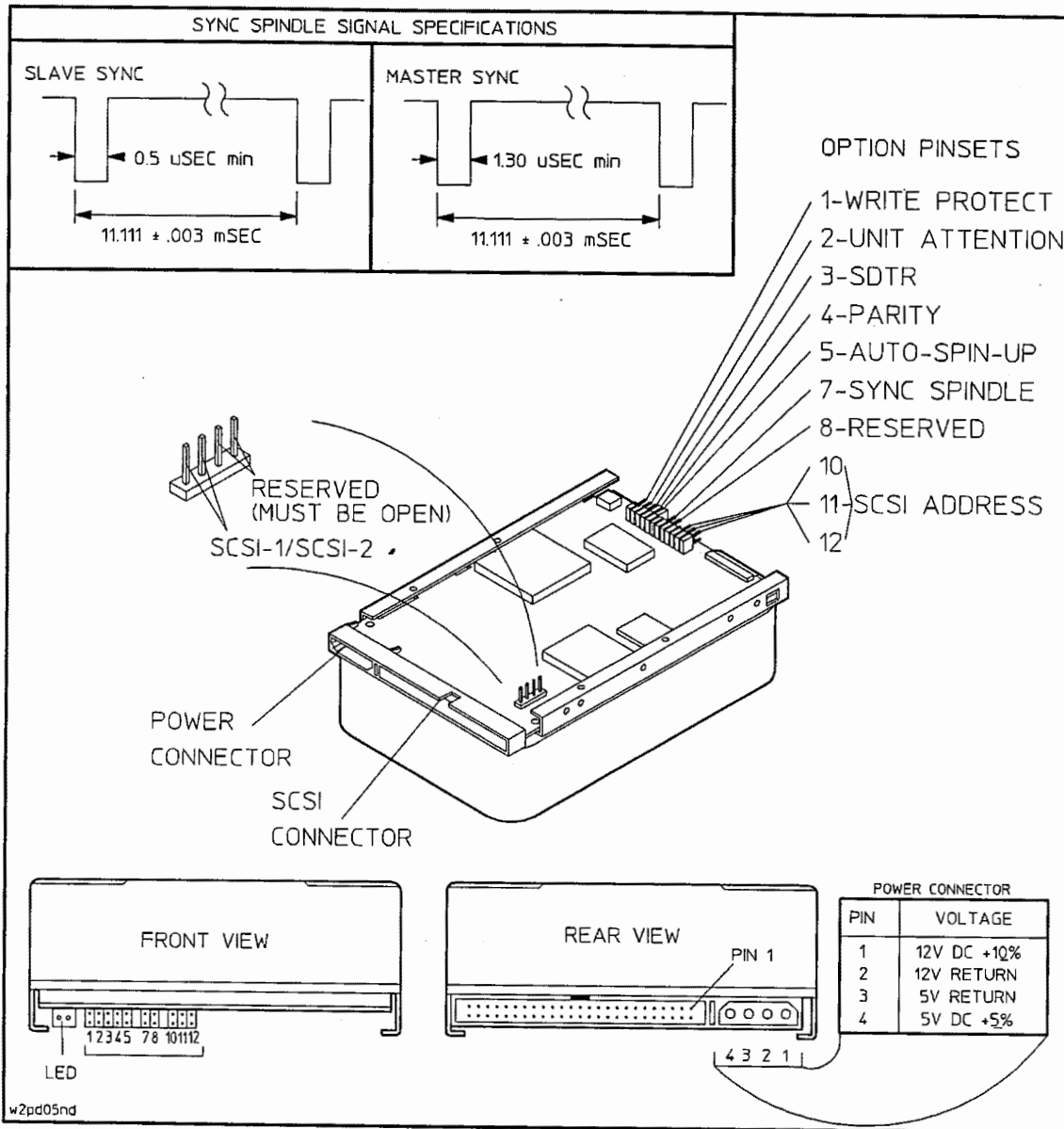
Figure F-2. Narrow, Differential: Interface, Address and Option Connectors
