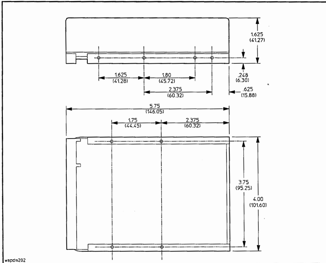
Figure F-1. Narrow, Differential: Disk Drive Dimensions and Mounting Locations
