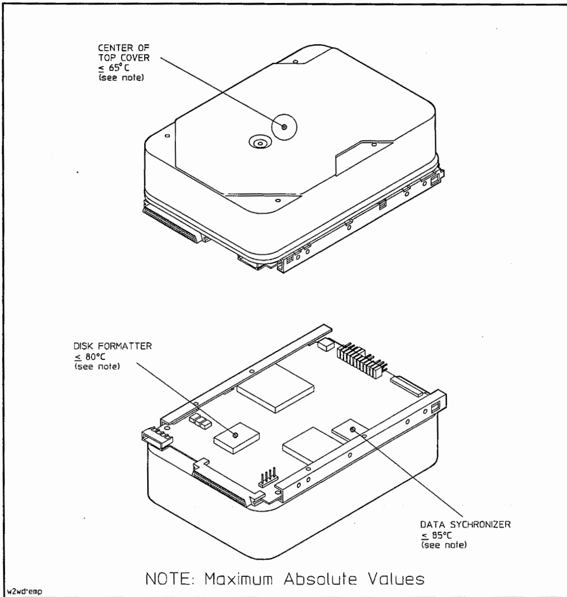
Figure G-4. Wide, Differential: Operating Temperatures
