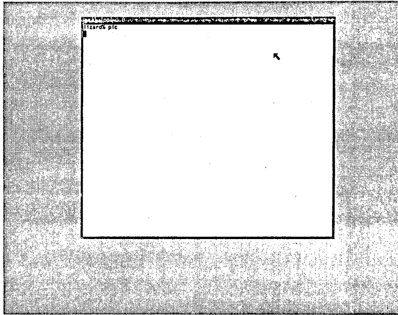
Figure 3-1: Sample Window
