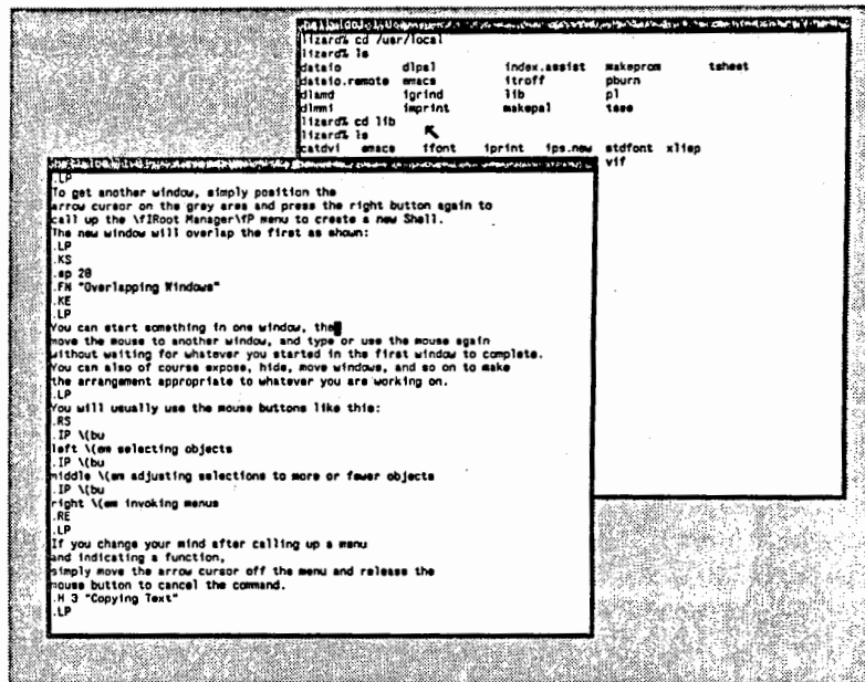
Figure 3-2: Overlapping Windows
