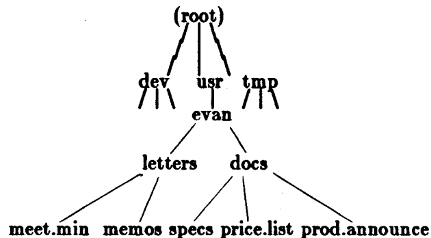
Figure 1-2: Sample File Hierarchy
