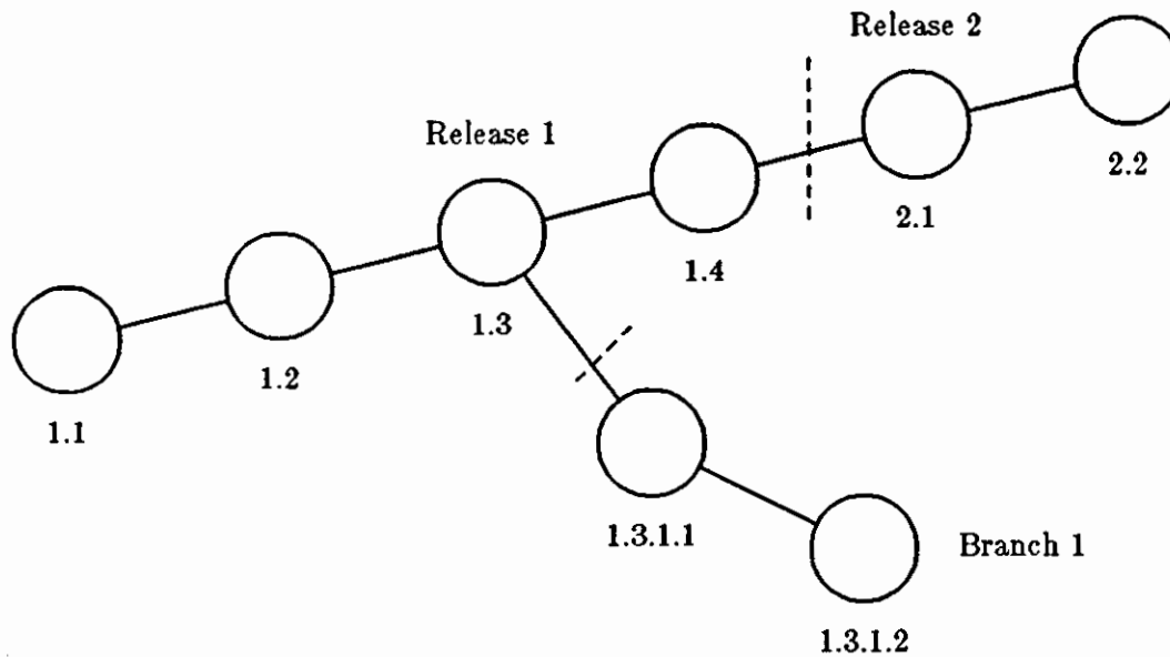
Figure 5-2: Tree Structure with Branch Deltas
