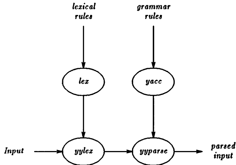
Figure 9-2: Lex with Yacc
