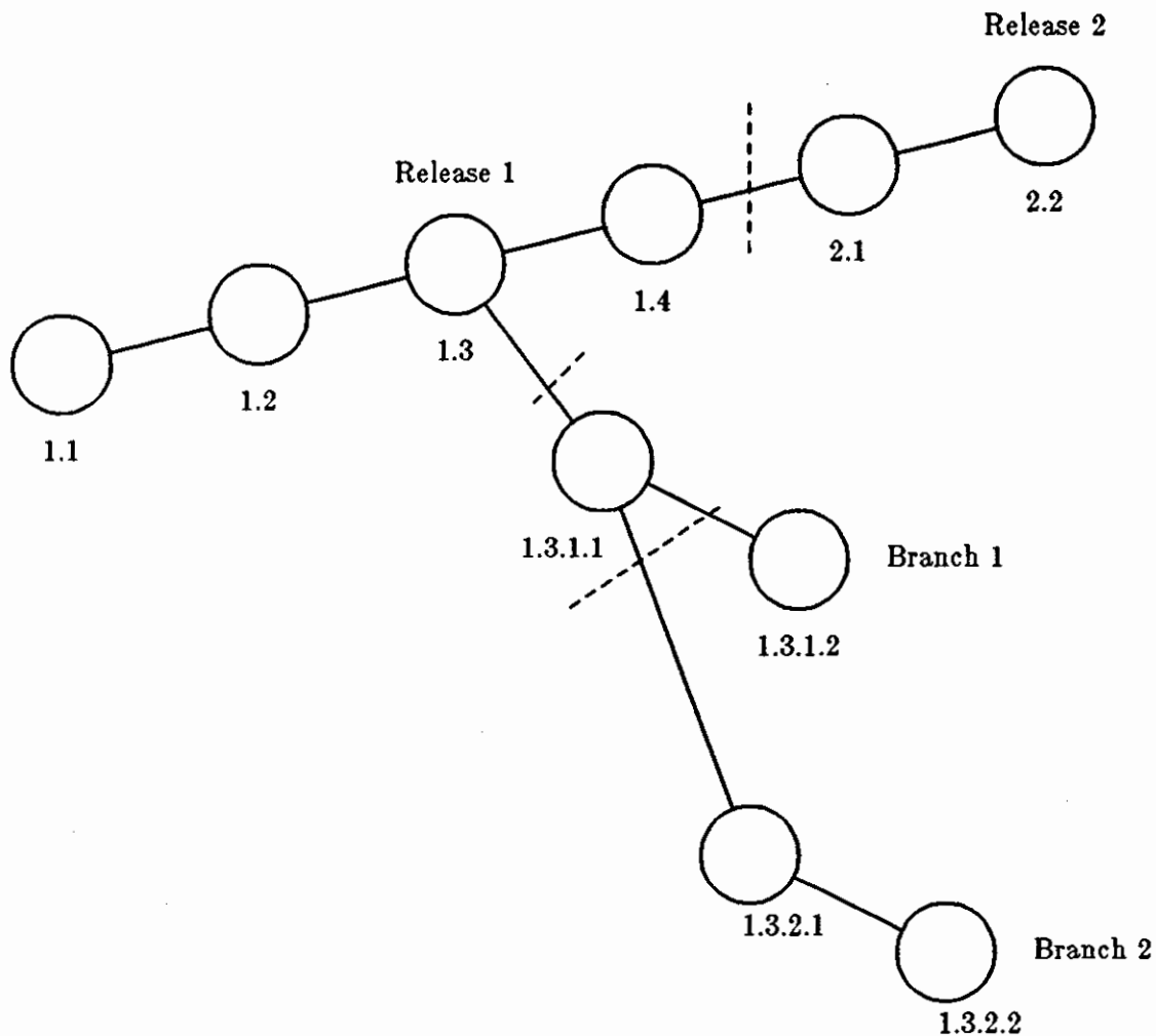
Figure 5-3: Extending the Branching Concept
