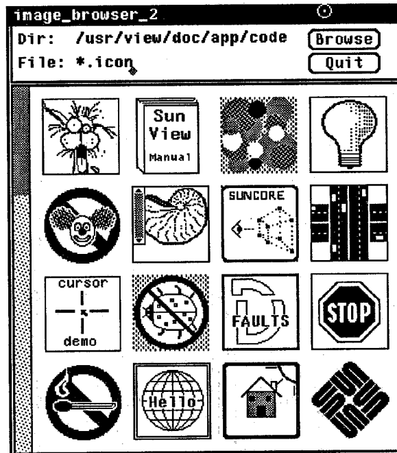
Figure 4-9 image_browser_2
