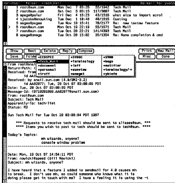
Figure 2-5 iconedit-menus
