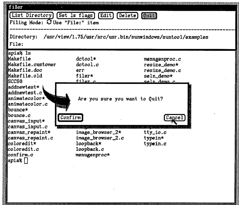
Figure 4-7 Pop-up Confirmer
