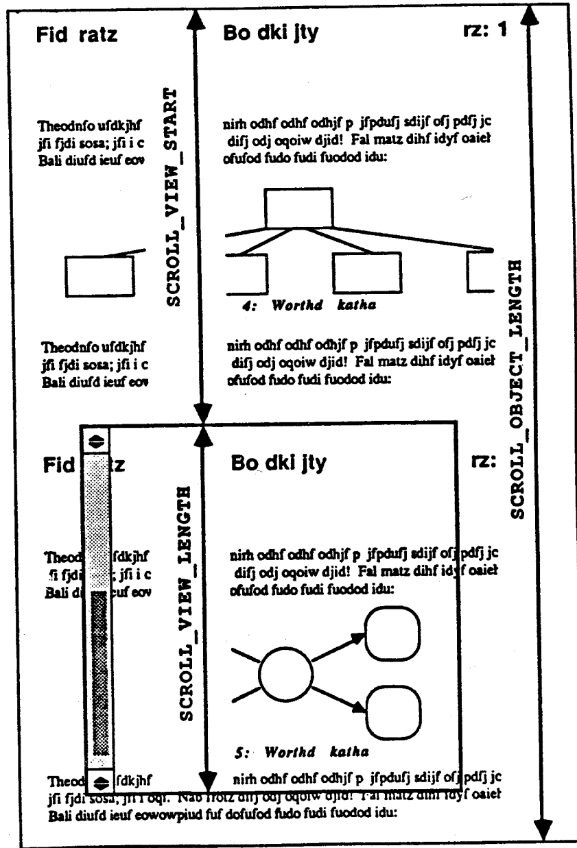
Figure 15-1 shows a two-page document being viewed within a window roughly half the size of the document. The three view-space attributes SCROLL_OBJECT_LENGTH, SCROLL_VIEW_LENGTH, and SCROLL_VIEW_START are shown superimposed on the document. Note the relative size and position of the bubble within the scrollbar — it is roughly half the size of the window and positioned near the bottom.
