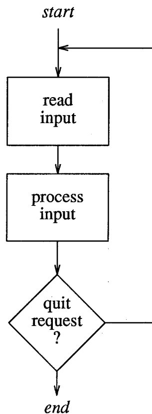
Figure 2-11 Flow of Control in a Conventional Program
