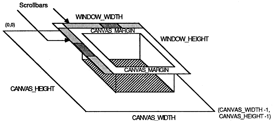
Figure 5-1 Canvas Geometry
