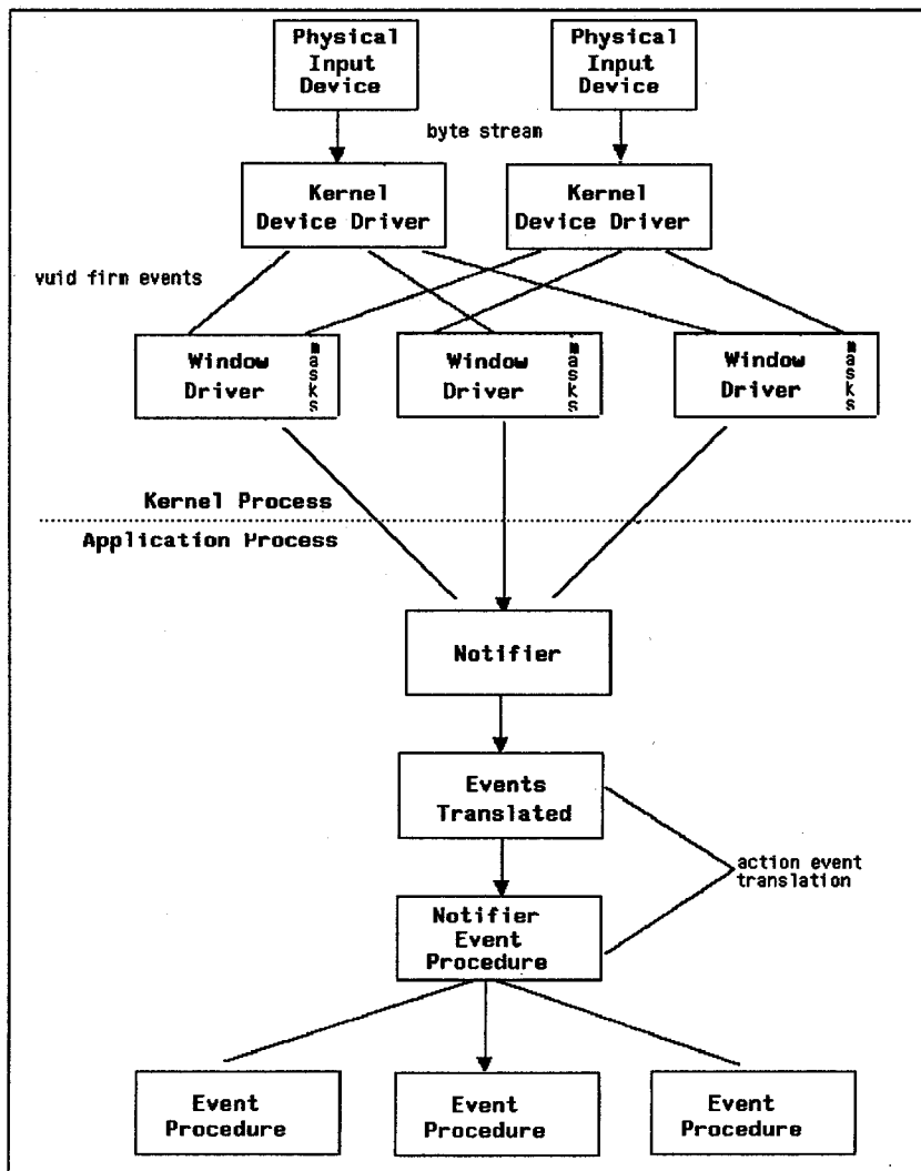
Figure 6-1 Input Events
