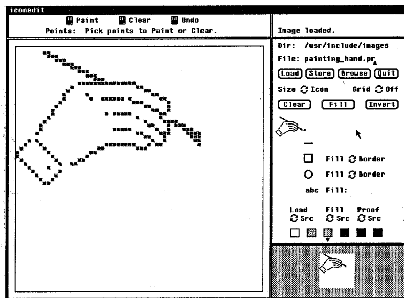
Figure 2-3 iconedit
