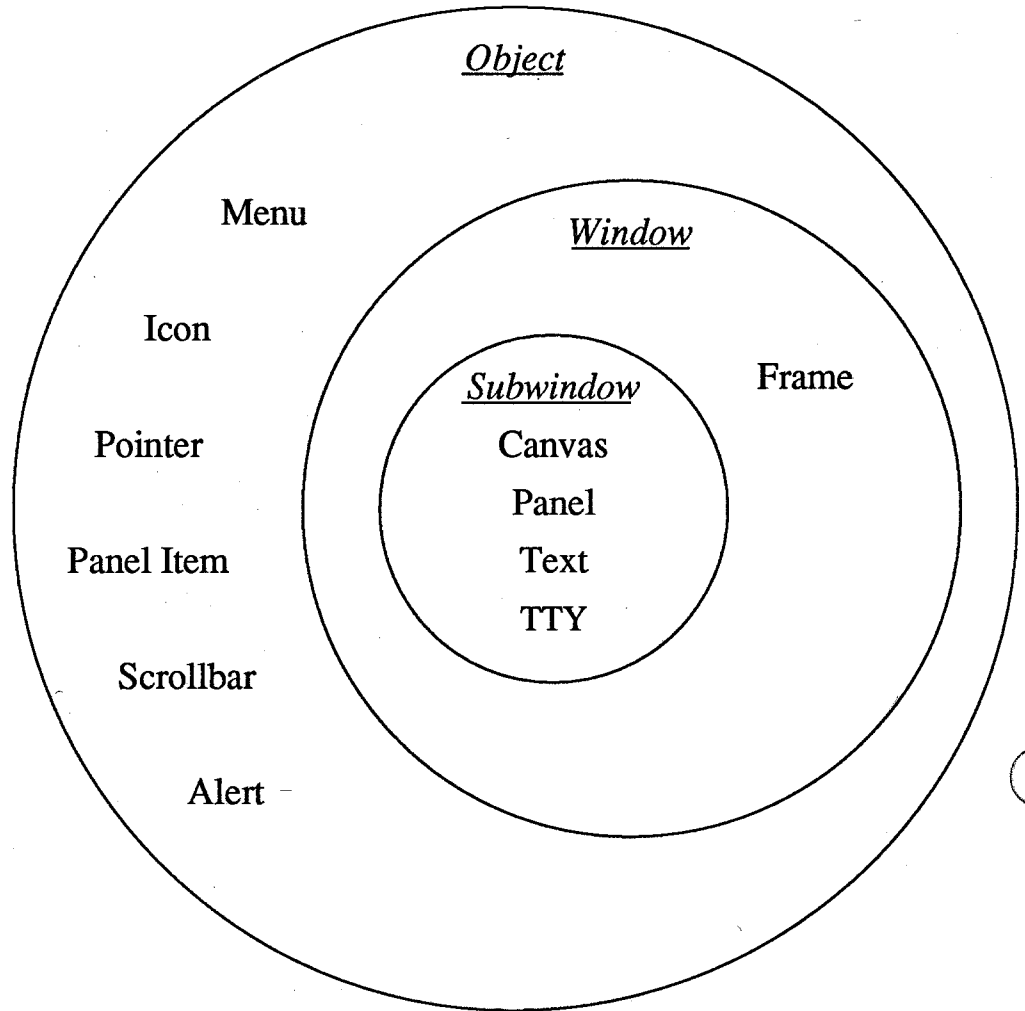
Figure 2-1 SunView Objects
