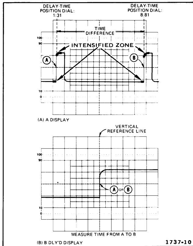
Fig. 27. Time difference between repetitive pulses.
